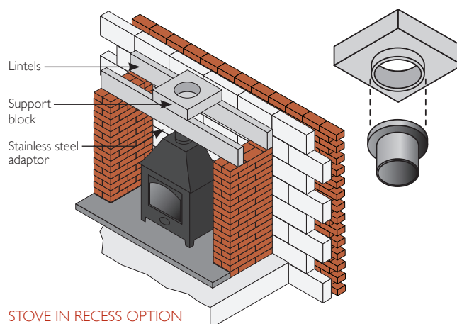
STOVE IN RECESS OPTION
