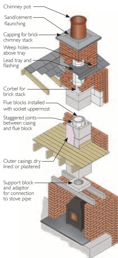
FREE STANDING STOVE IN A RECESS.
