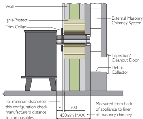
REAR OUTLET TWIN WALL CONNECTING FLUE PIPE INTO EXTERNAL MASONRY CHIMNEY THROUGH A WALL
