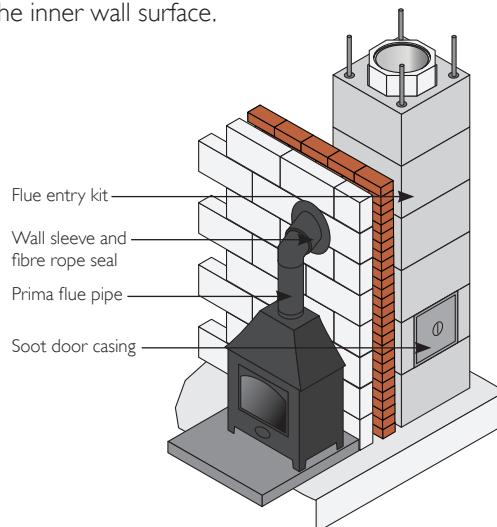
FREE STANDING STOVE OPTION
