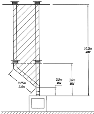
Vertical from the top of the appliance
