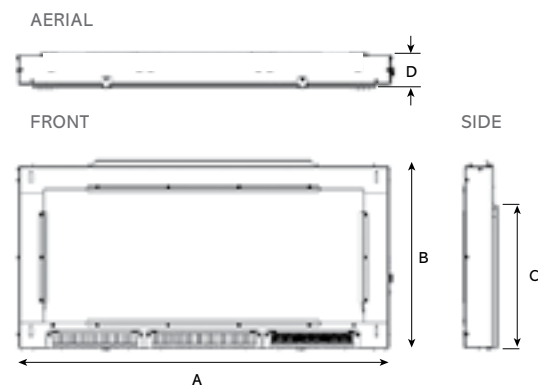
Studio Electric Fire Dimensions (mm)
